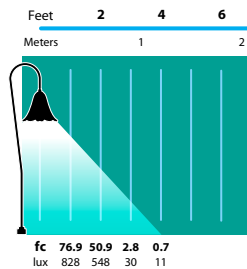
PL-04 Half Spread Photometrics 8 ft. (2.4m) diameter
